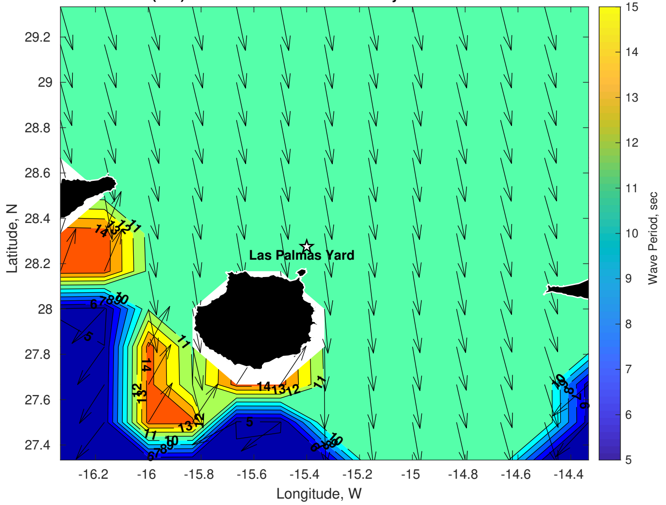
Wave Period (sec) for Las Palmas Yard at 03-May-2024 06:00:00
