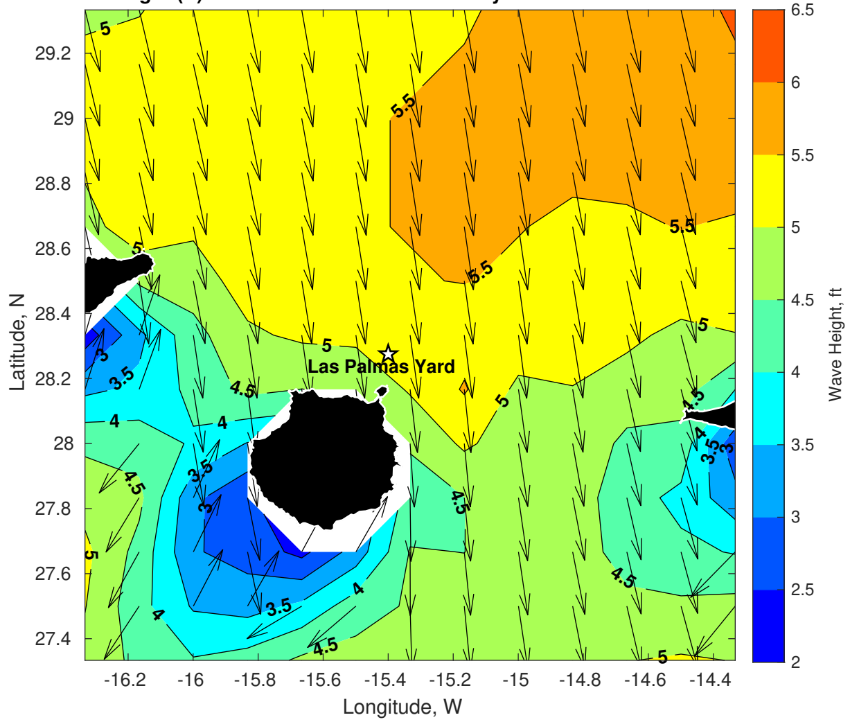
Wave Height (ft) for Las Palmas Yard at 03-May-2024 06:00:00
